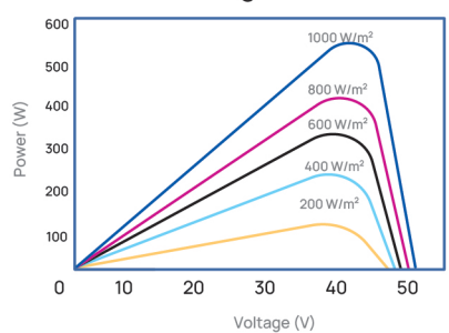
Power-Voltage Curve 555W
